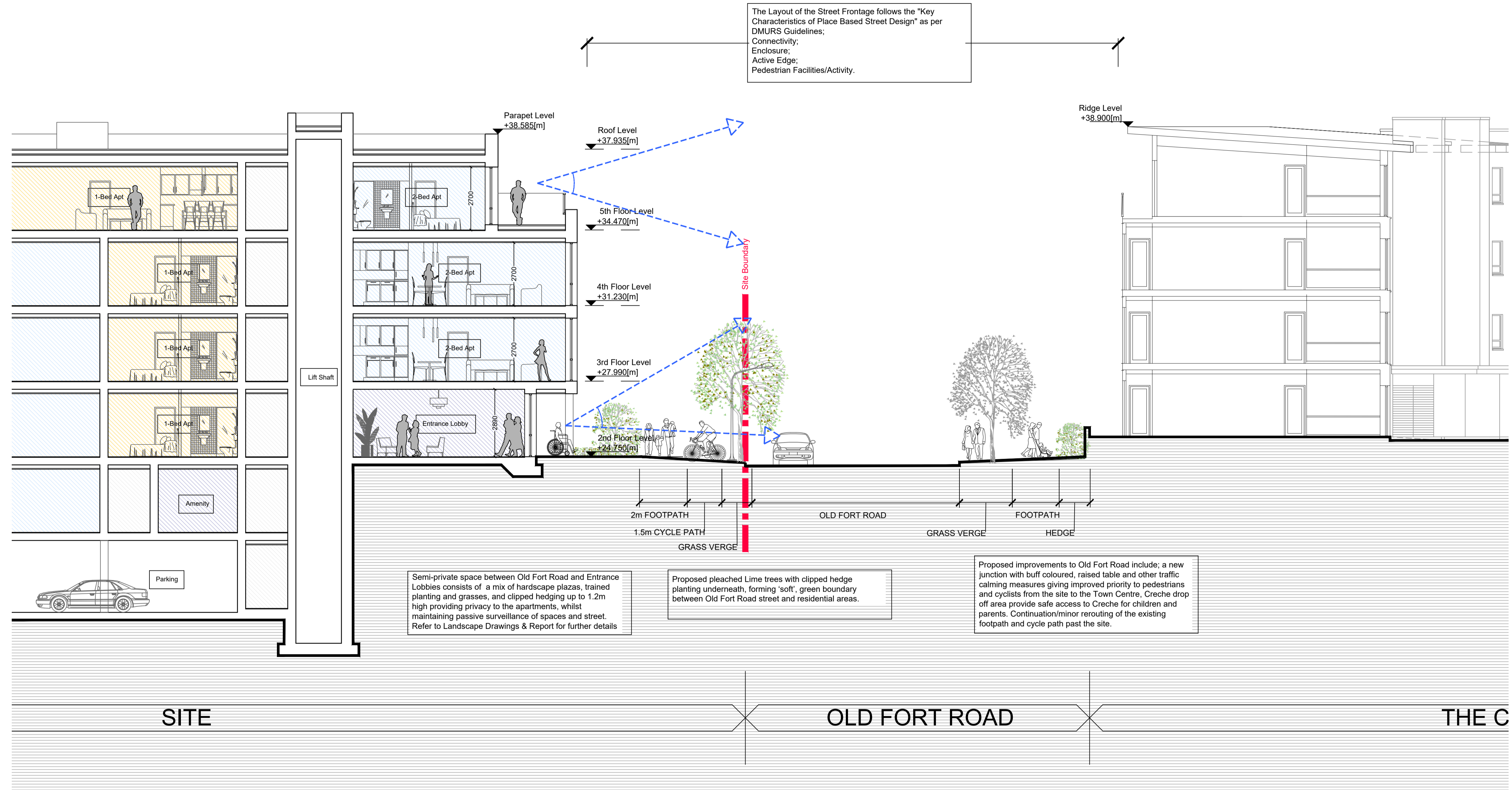
BLOCK B - Cross Section through Old Fort Rd Scale 1:100
