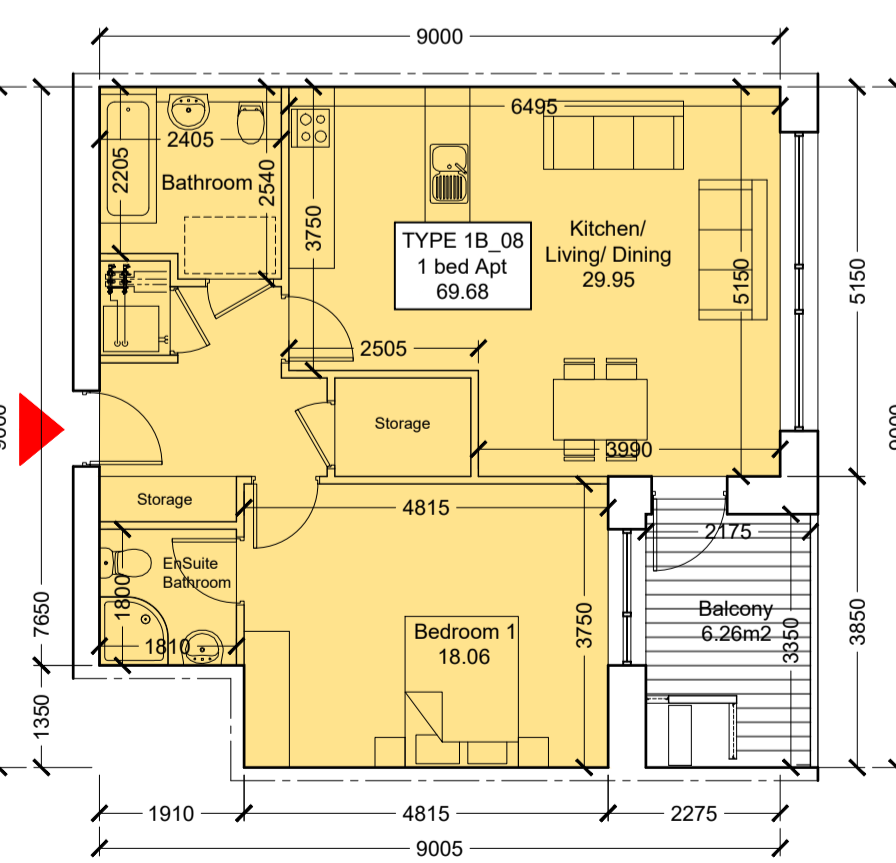
Type 1B_08 Scale 1:100
