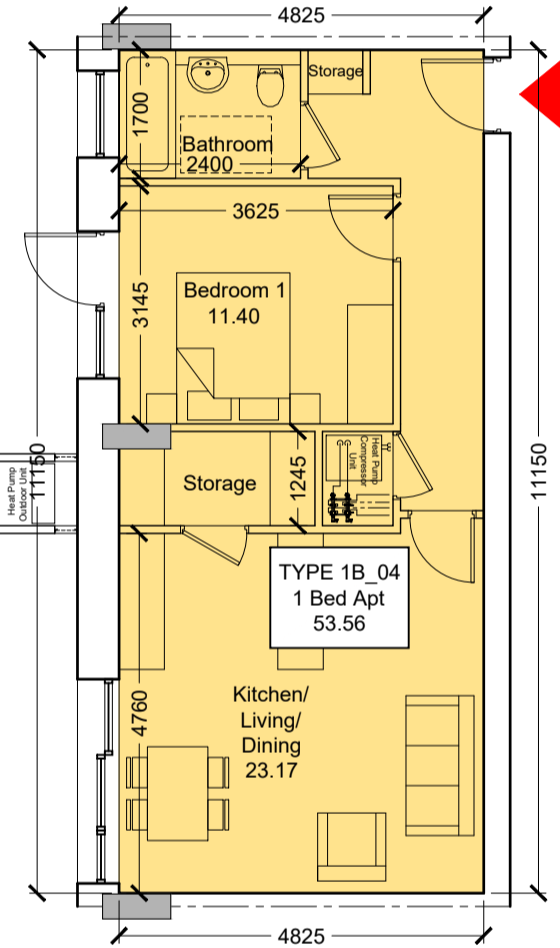
Type 1B_04 Scale 1:100
