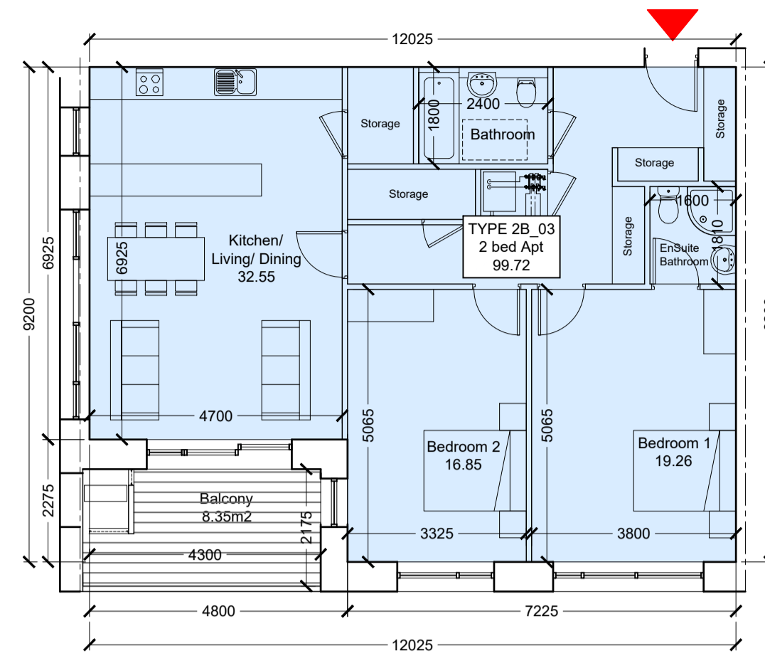
Type 2B_03 Scale 1:100
