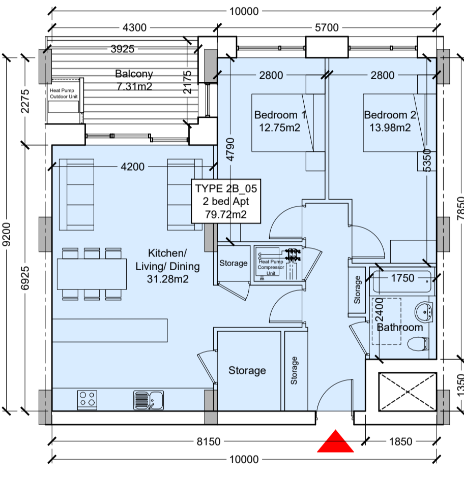
Type 2B_05 Scale 1:100
