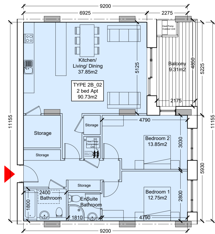
Type 2B_02 Scale 1:100
