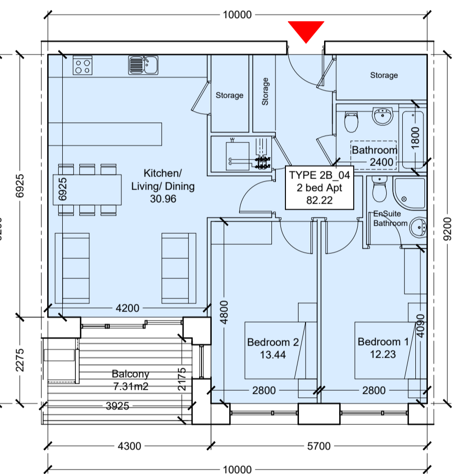
Type 2B_04 Scale 1:100
