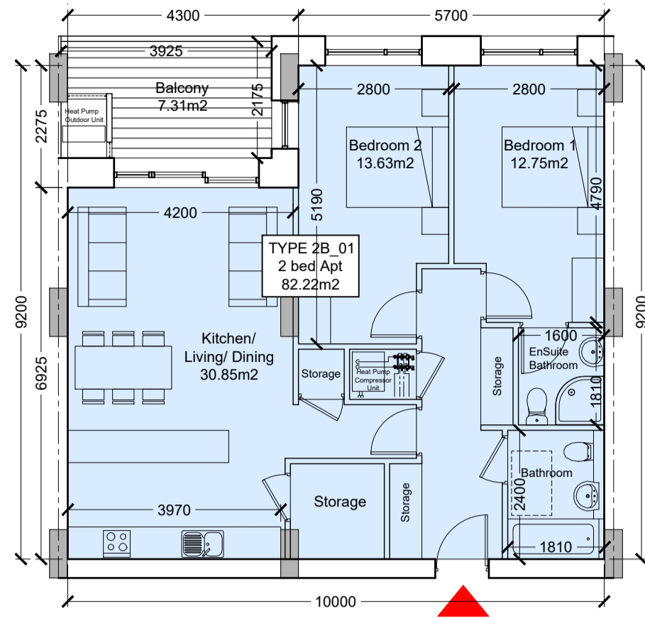
Type 2B_01 Scale 1:100
