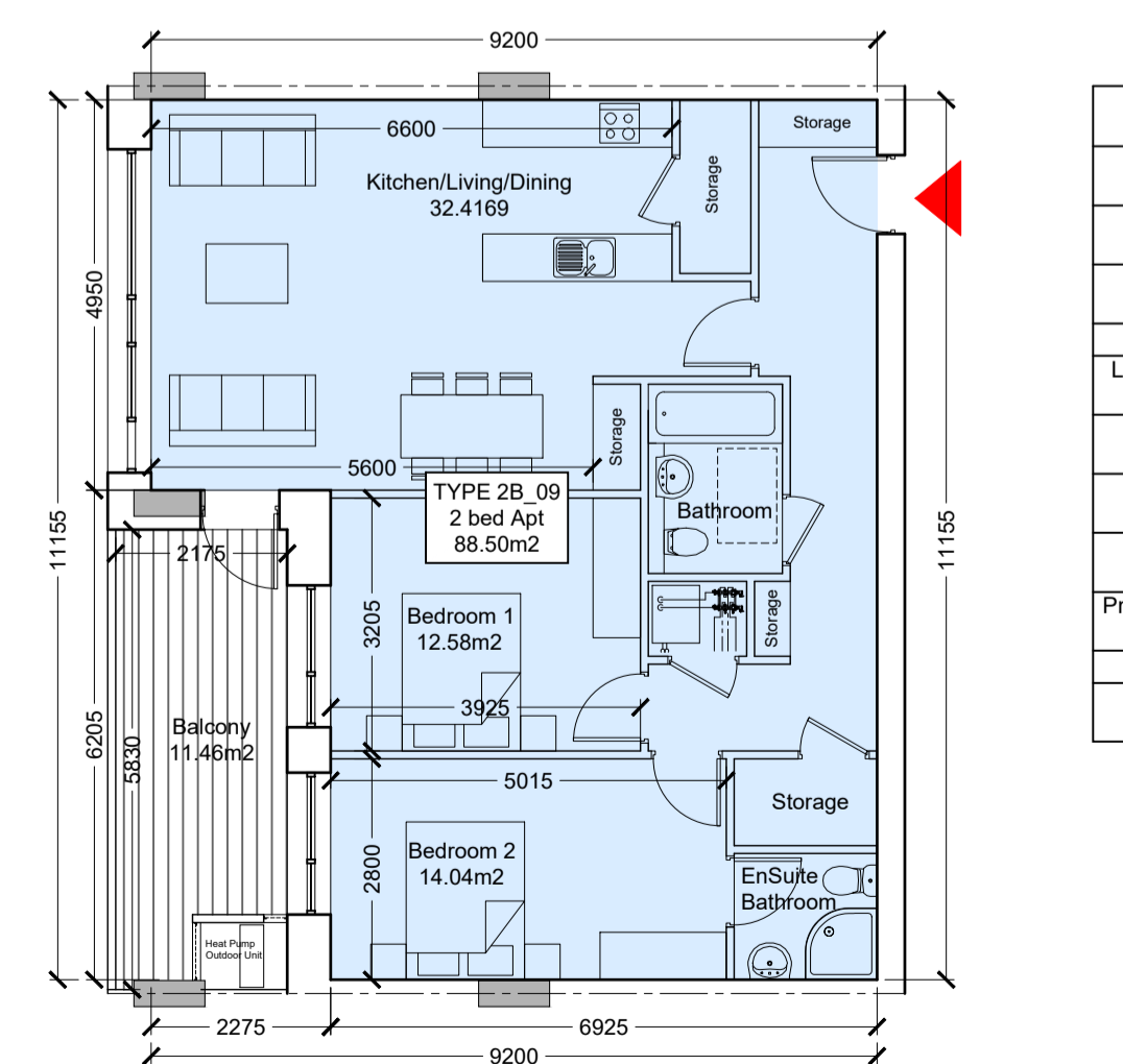
Type 2B_09 Scale 1:100
